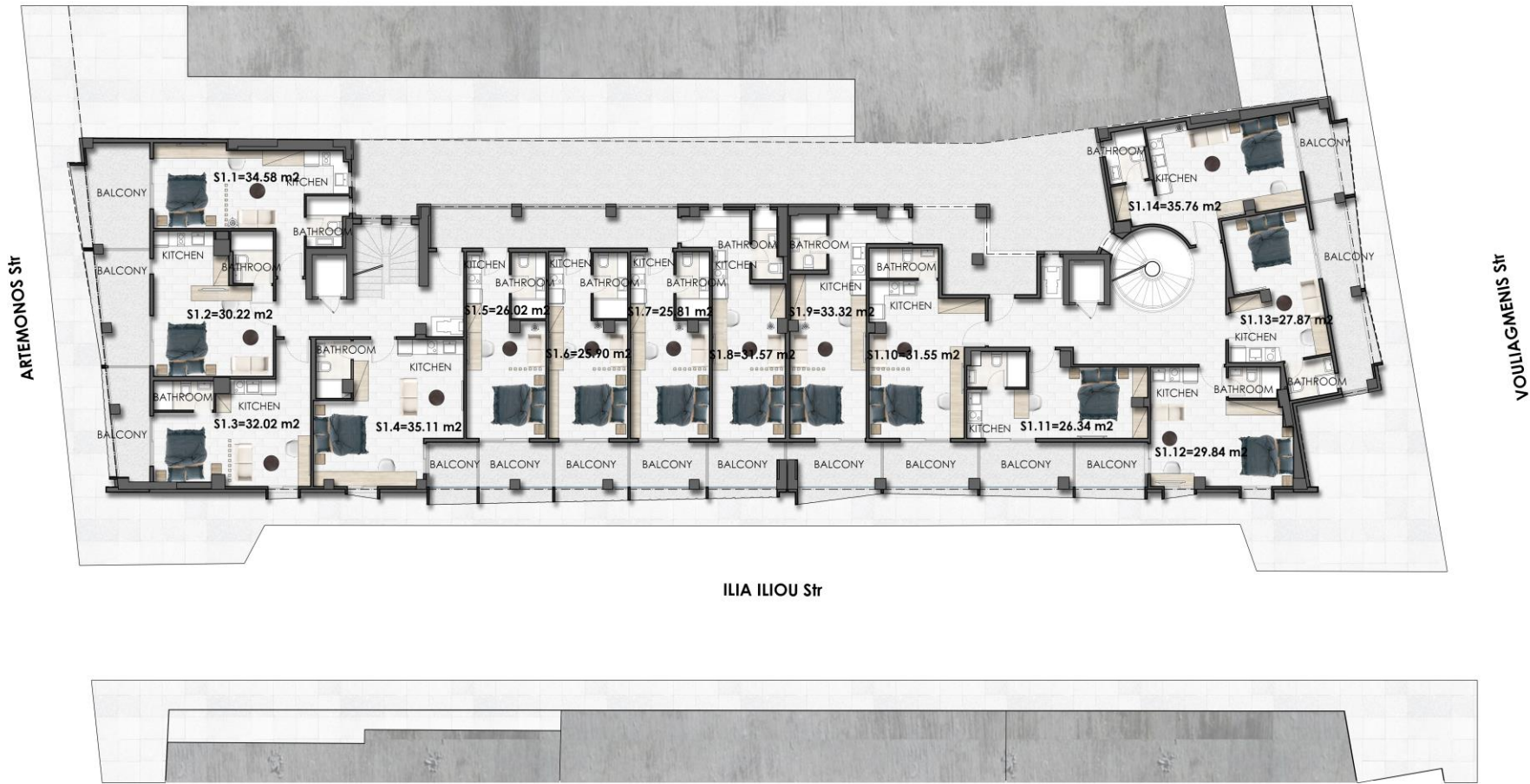
FIRST FLOOR
